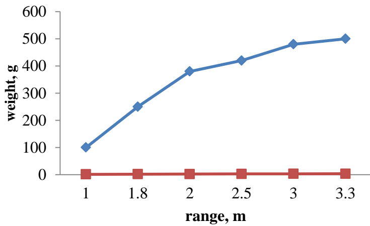
Figure 2. Defining of propellant properties of gas-generator compositions № 1 depending on mass of pyrotechnic compounds
