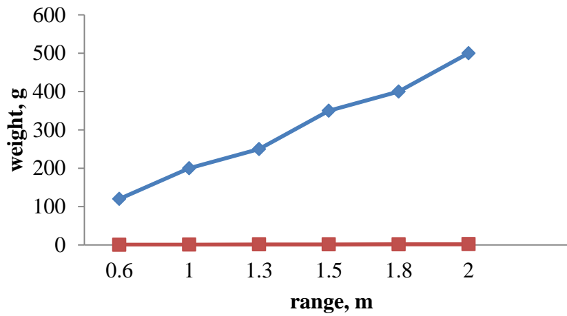
Figure 2. Defining of propellant properties of gas-generator compositions № 1 depending on mass of pyrotechnic compounds
