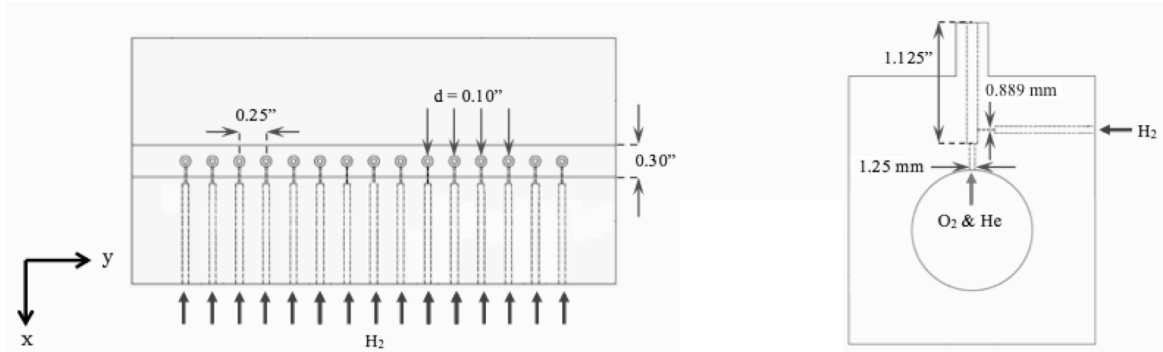
Figure 2. University of Maryland LMDE Geometry. Left: View of the LMDE looking down into the XY plane. Right: View of the LMDE looking end on at the XZ plane.
