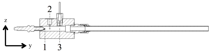
Figure 1. Cross-section view of the PDE. Positions 1, 2, and 3 correspond to the spark ignition source, location of gas injection, and an upstream Kistler transducer placement, respectively. Flow is in the positive Y-direction. The X, Y, and Z-axes form a right-handed coordinate system.
