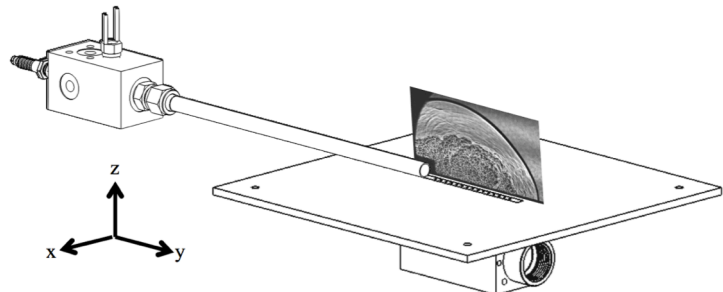
Figure 3. Diametric view of the PDE and LMDE assembly. Blast waves and cross-flows propagate in the positive Y and Z directions, respectively. Shadowgraph images are of the YZ plane as shown.
