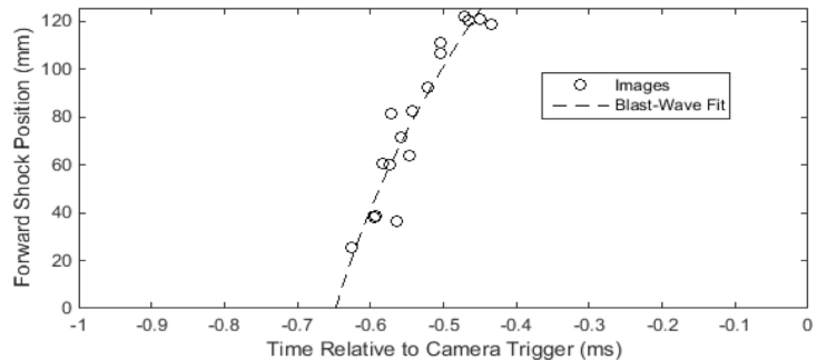
Figure 5. Forward position of the blast wave correlated with the relative image acquisition time.
