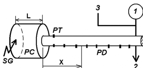
Figure 1. Schema of the experimental setup. PC – prechamber, SG – spark gap, PT – pressure transducer, PD – photodiodes, X – distance along the channel, L – length of the prechamber, 1 – manometer, 2 – pumping system, 3 – mixture filling system.
