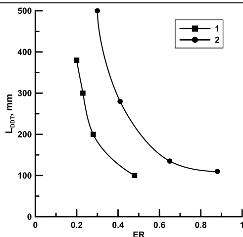
Figure 3. Pre-detonation distance in dependence on ER for push-effect detonation initiation. 1 – acetylene-oxygen mixture, 2 – propane-butane-oxygen mixture.
