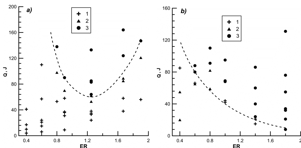
Figure 4. Map of direct detonation formation in dependence on energy, released in the prechamber, and ER of mixture. a, propane-butane-oxygen; b, acetylene-oxygen. 1, no direct formation; 2, formation of detonation between 10 and 40 tube diameters; 3, direct formation.
