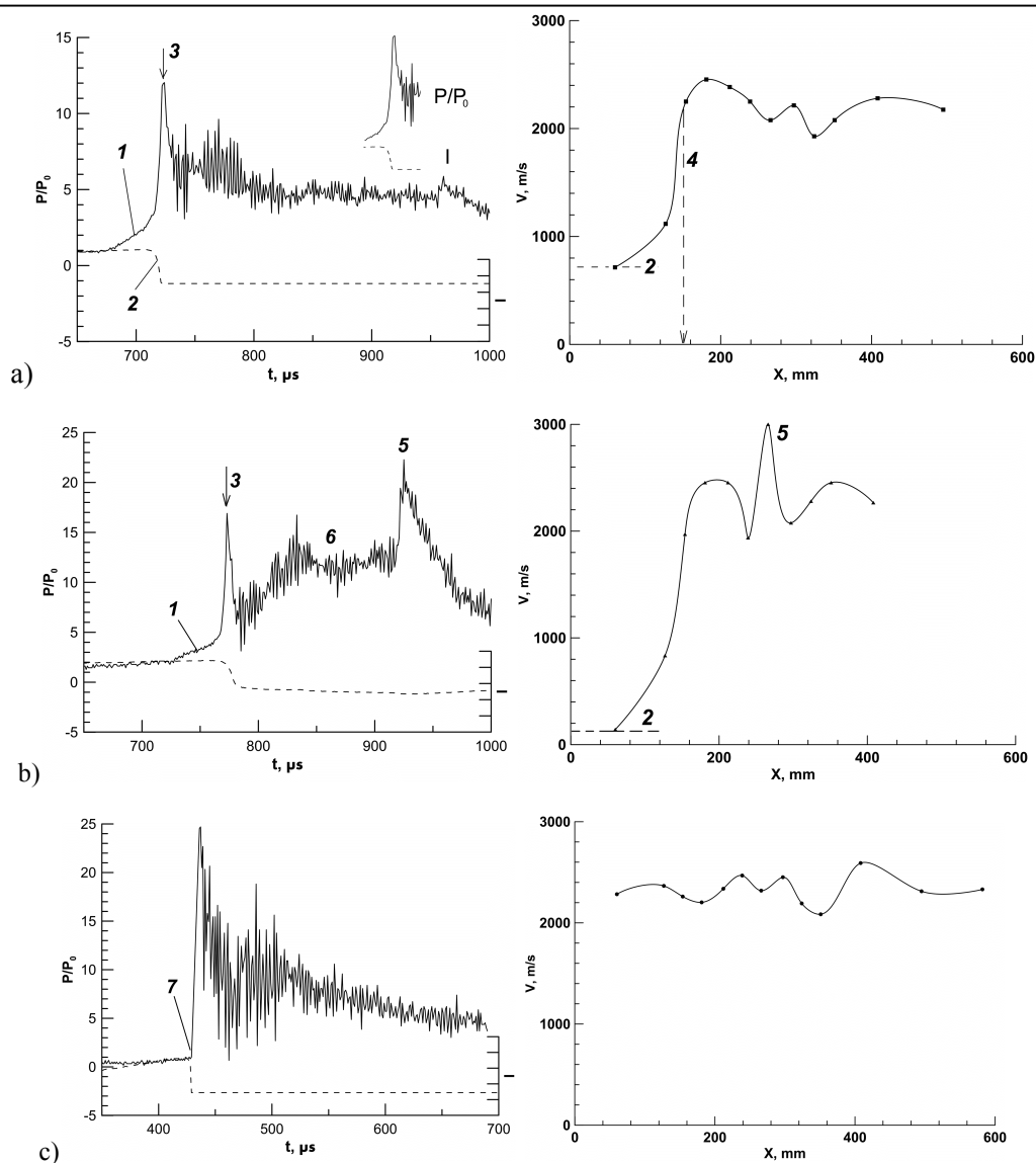
Figure 2. Readings of pressure transducer ( P/P_0 , up) and photodiode ( I , r.u., down) at the position of 10 tube diameters from the beginning of the channel and evolution of the velocity of the flame front along the axis of the channel. Prechamber diameter/length: a, 10/7 mm; b, 20/8 mm; c, 10/20 mm. 1 – increase in pressure due to compression waves, 2 – flame front and flame front velocity, 3 – pressure peak due to flame front, 4 – pre-detonation distance, 5 – pressure/velocity peak due to superposition of waves, 6 – steady in pressure due to combustion products, 7 – detonation wave.
