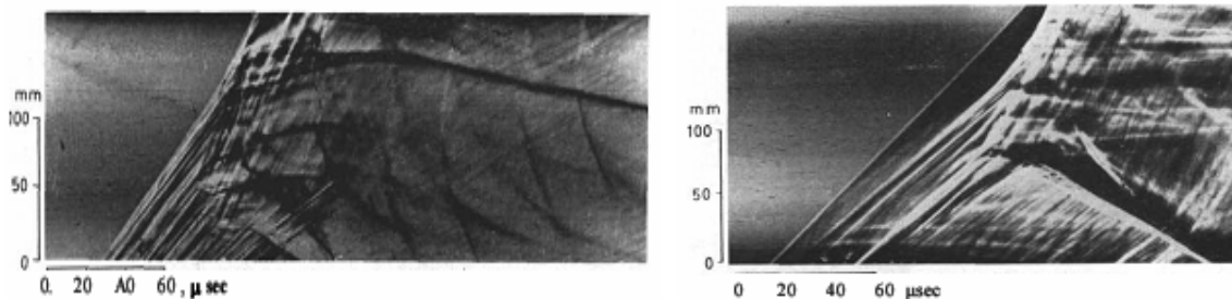
Figure 2. Soloukhin's Schlieren streak images of detonation formation in mixture of natural gas and oxygen (left) and in hydrogen-air mixture (1958).
