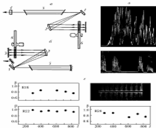
Optical scheme of the Soloukhin-Yakoby laser spectrograph, typical records, and measurement results on vibrational levels population [19].
