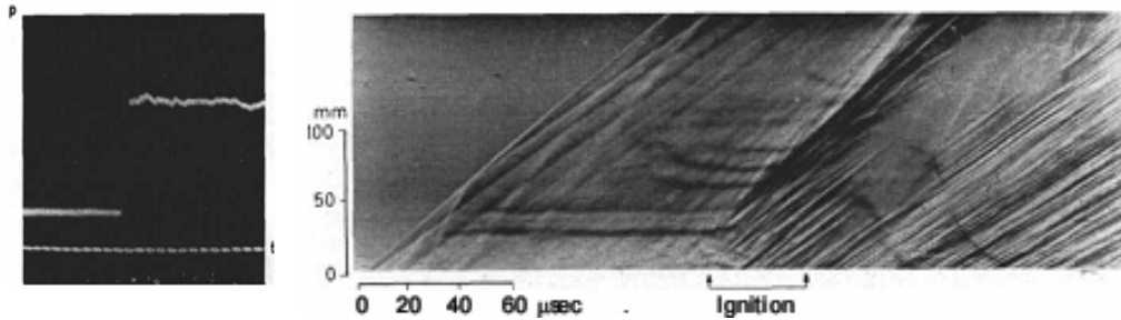
Figure 1. Soloukhin's pressure record in shock wave and Schlieren streak image of ignition initiation behind the shock wave in a mixture of natural gas and oxygen (1957).
