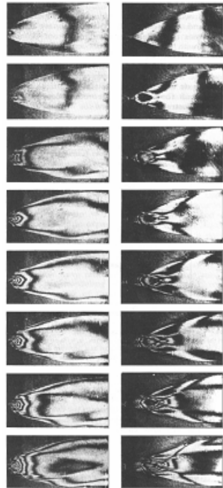
Michelson interferometer frame records of starting processes in mixing gasdynamic lasers [17]. Time interval between frames is varied up to 1 \mu s.
