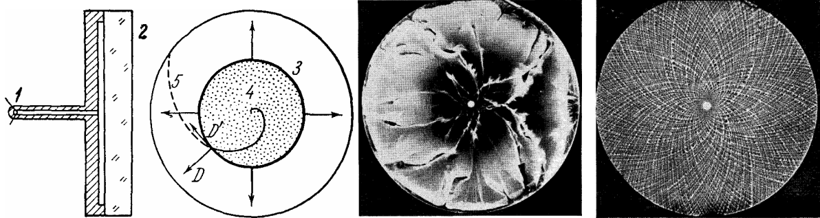
Figure 3. Diagram of the experiment for the study of the structure of a cylindrically expanding detonation front (left): (1) Detonation tube with contacts for ignition; (2) transparent surface of the explosion duct; (3) detonation front; (4) combustion products; (5) trajectory of the transverse wave. The arrows indicate the normal and tangential velocity components of the transverse wave. In the center and on the right are Soloukhin's photographs of a detonation for a decaying and non-decaying detonation in a C_2H_2+O_2 mixture [4] (1959).
