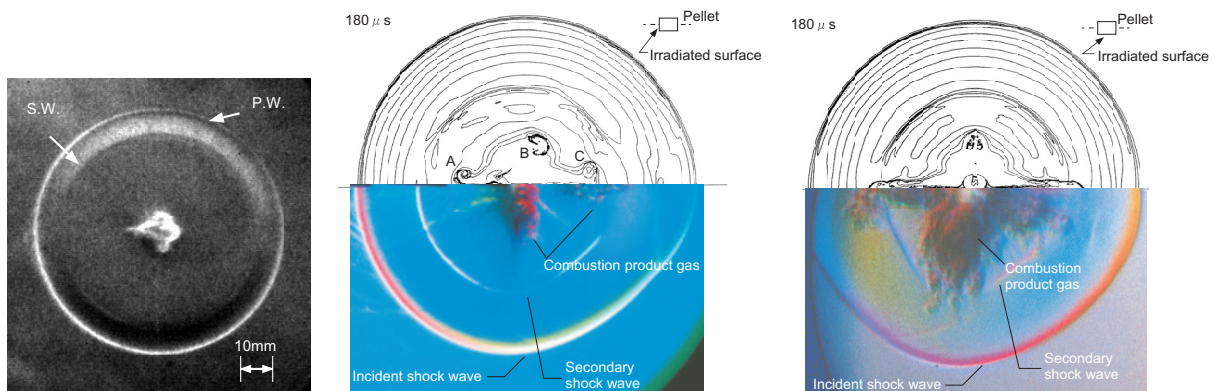
Fig. 4 Shock wave generated by 0.5mg silver-azide charge
