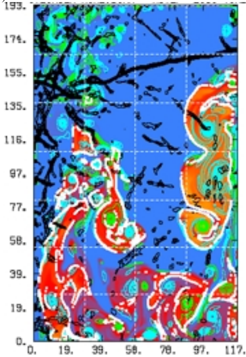
Figure 1. AMR simulation of the explosion of a 875-g cylindrical TNT charge in a 16.6\text{-m}^3 chamber filled with air at atmospheric pressure. TNT detonation products (shown in yellow ), mix with air (depicted as blue ) thereby forming combustion products (represented as red ). Exothermic cells are marked by white dots. Vorticity contours are green (negative) and turquoise (positive), while dilatation contours are black .
